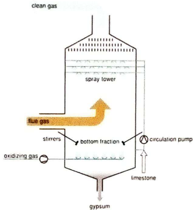
Fig 1 : Wet Scrubber Meachanism
