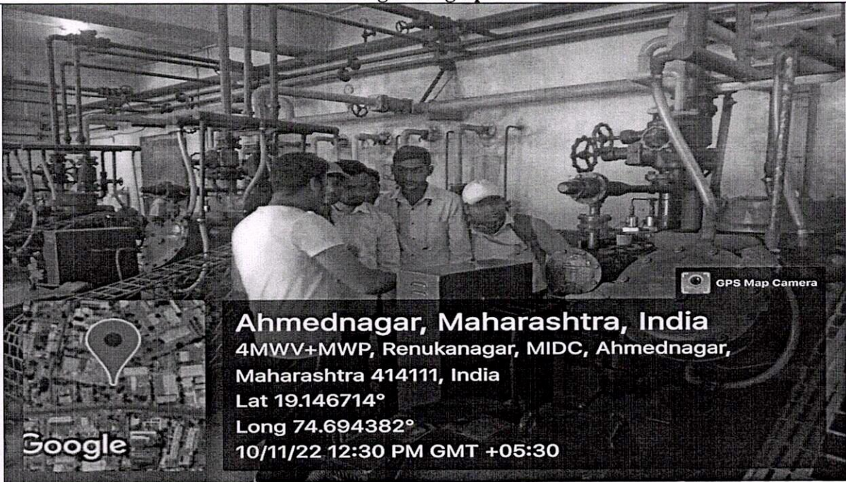
Compressor Room
