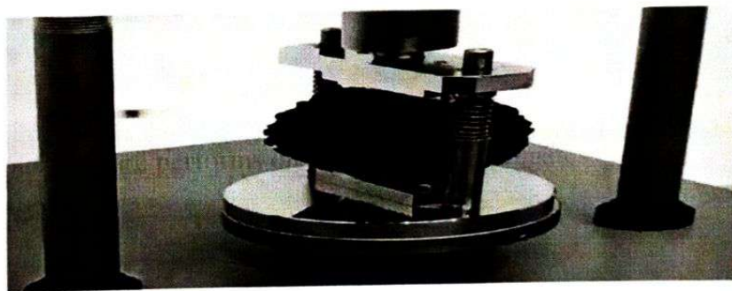
Fig : bitumen specimen in marshall stability apparatus mold
