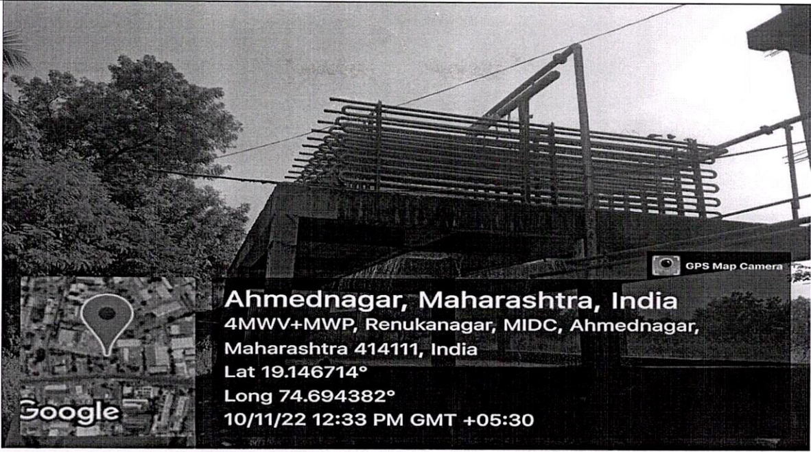
Evaporative Condenser
