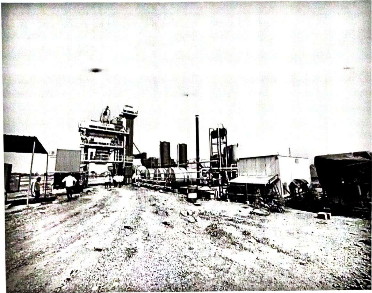
Image : GHV india private limited , bitumen hot mix plant
