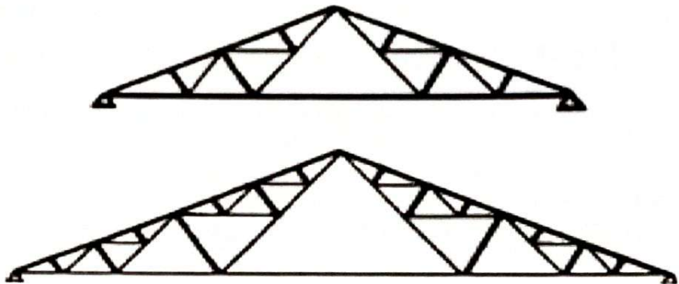
Fig: - Belgian truss.
