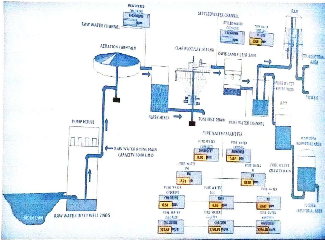
M.L.D.C. NAGAR WATER SUPPLY FLOW DIAGRAM
